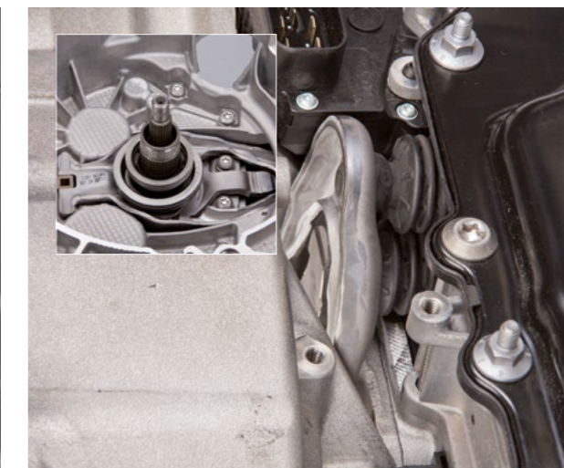
Engagement lever made from sheet steel – transmission construction date from June 2011, 2nd generation OAM and OCW
