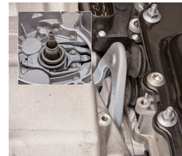
Cast engagement lever – transmission construction date up to May 2011, 1st generation OAM
