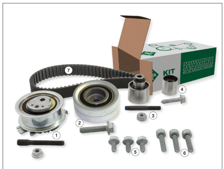
Fig. 1: INA-spanrol KIT 530 0550 10
