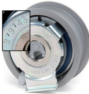
Photo 1: 531 0777 10 – Old tensioner pulley (979743)
