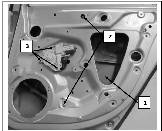
Porta lato destro, Portière arrière droite, Right rear door, Puerta lado derecho, Hinten rechte Tür, Porta traseira direita, Sag arka kapi, νόρτα οπισθια δεξιά
